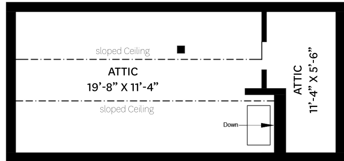
ATTIC FLOOR PLAN Ceiling Height: 5'-5"
